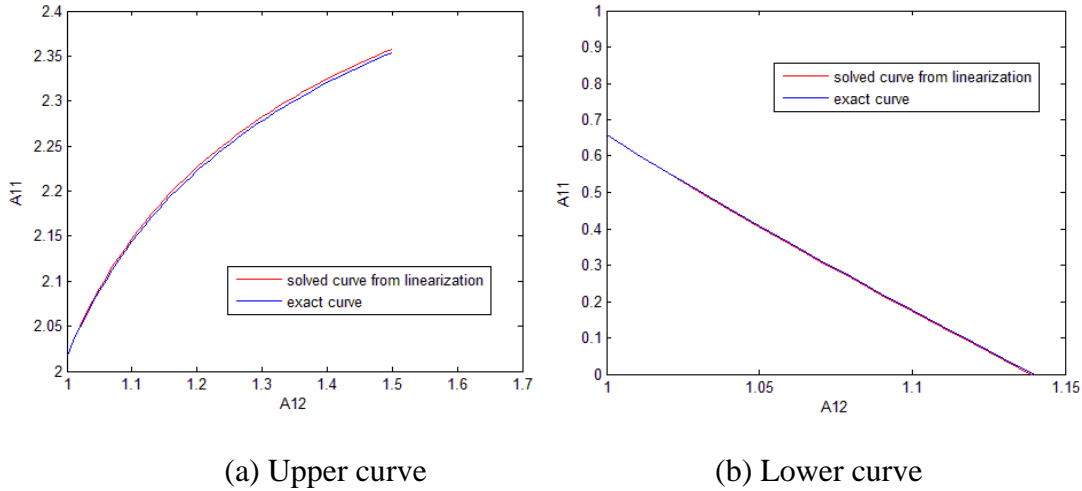
Figure 6.5 Profiled curve from linearization method
