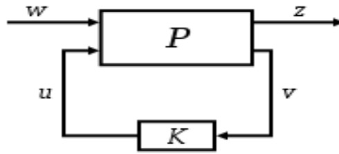
Figure 3.3 H_2/H_\infty Method
